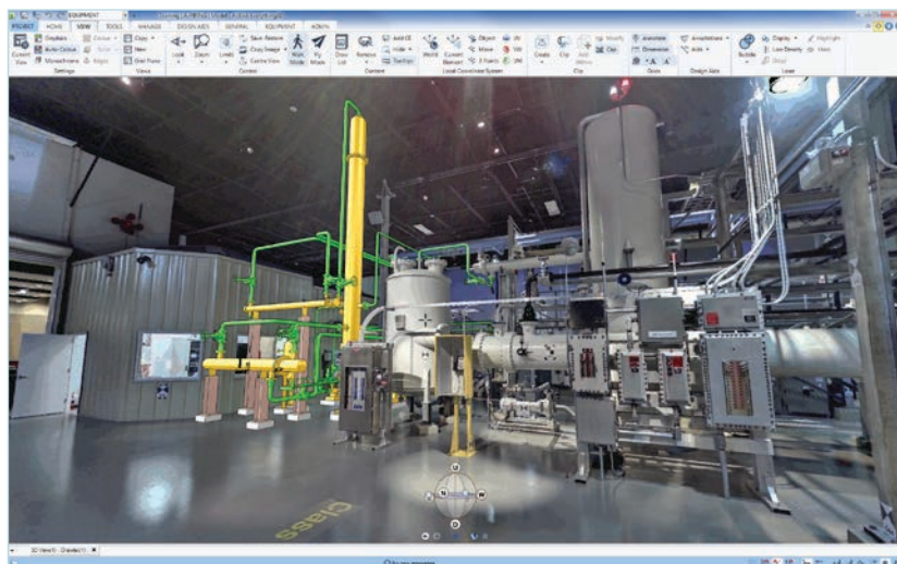
Laser scan data integrated into the 3D view
