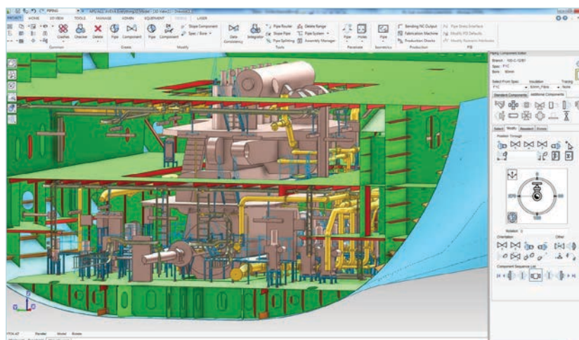
Hull data in the 3D view
