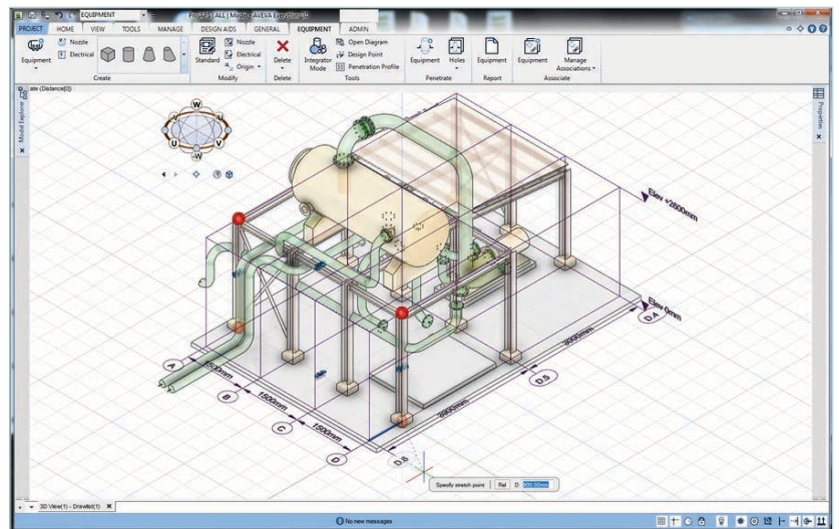
Grid lines, dimensions and annotations can all be included in the 3D view
